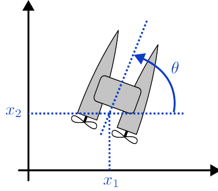
Figure 4.2 – Dubins car
