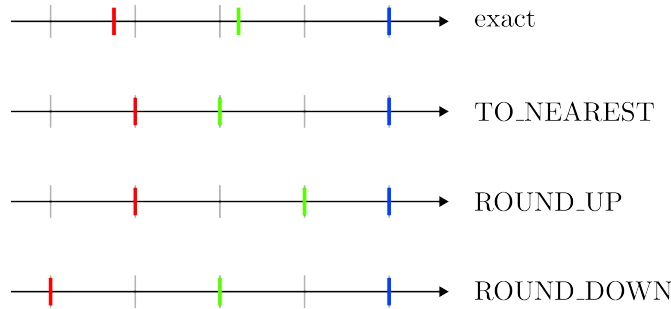
Figure 9.1 – Rounding strategies
