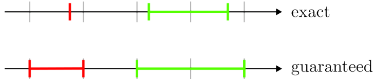
Figure 9.2 – Guaranteed computer representation of real numbers and intervals
