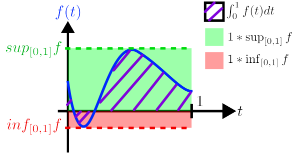
Figure 8.8 – Riemann integrals
