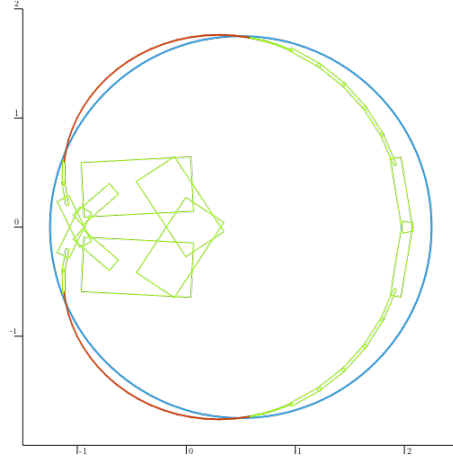
Figure 7.19 – Output of the Ad-PEIBOS algorithm
